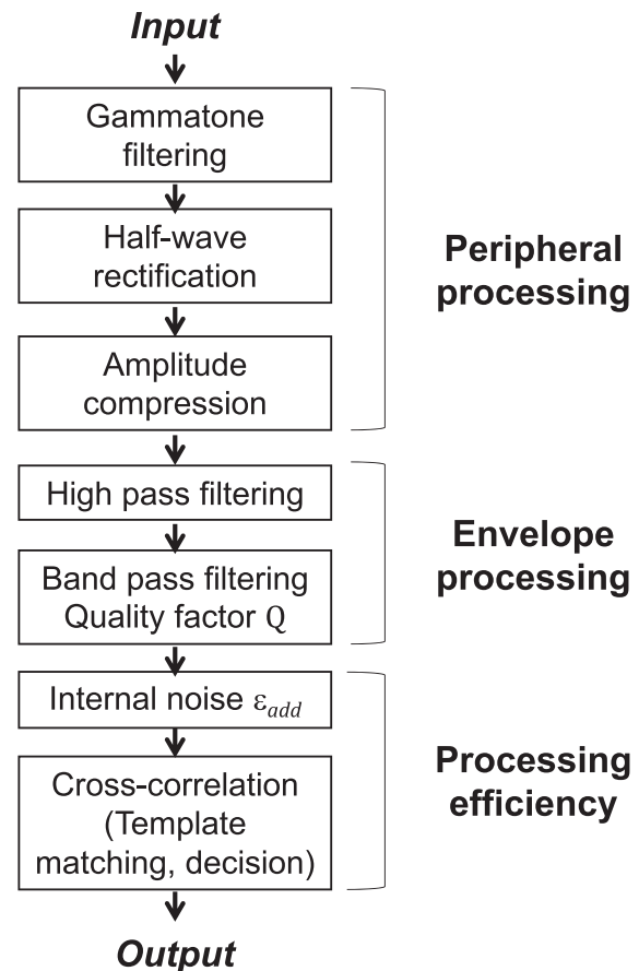
FIG. 3. Schematic representation of the computational model of AM processing.
